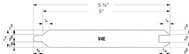
Cayaki V-Joint Siding Profile
