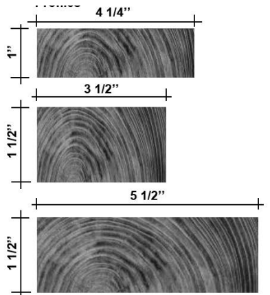
Western Red Cedar Moulder Profiles
